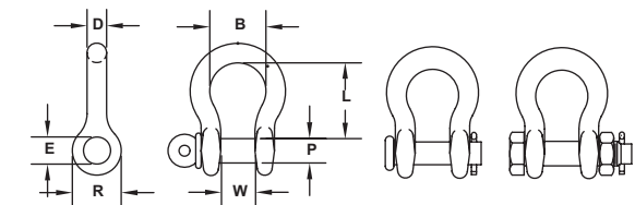
Screw Pin
