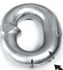
Figure 2: Location of nicks, gouges, and notches will dictate their severity.
