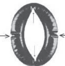
Figure 5: The tube "under load" shows wrinkles in the areas of compression.
