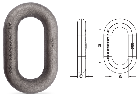
Keeper Link
